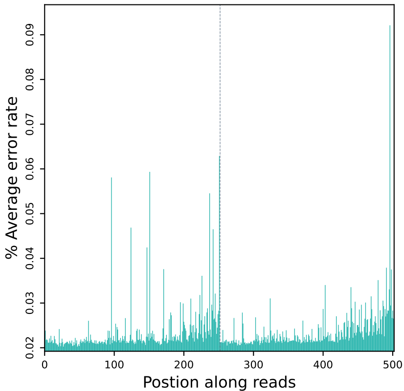
Error rate distribution along reads (R10417)
